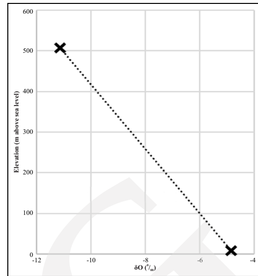
Figure 3. Interpolation between the elevation of the rainwater sampling point and the \delta^{18}\text{O} value.
