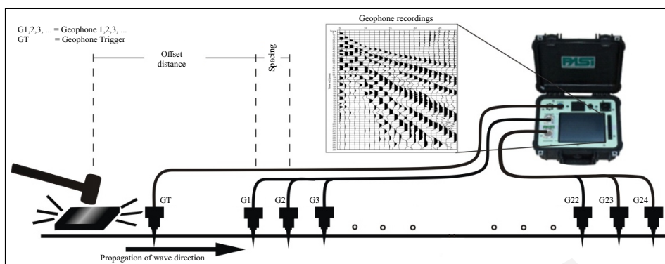
Figure 2. MASW data measurement configuration in the field using Seismograph PASI Mod. 16S24-P s.n. 121217044 (modified from (Rusdy et al. , 2016).
